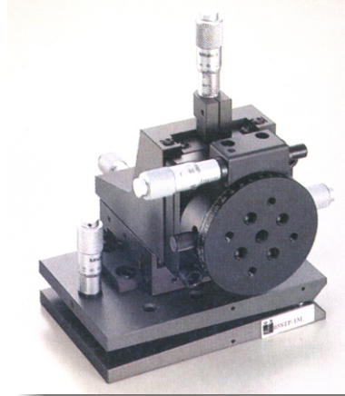
X, Z, \theta_z , \alpha Axis 軸座
