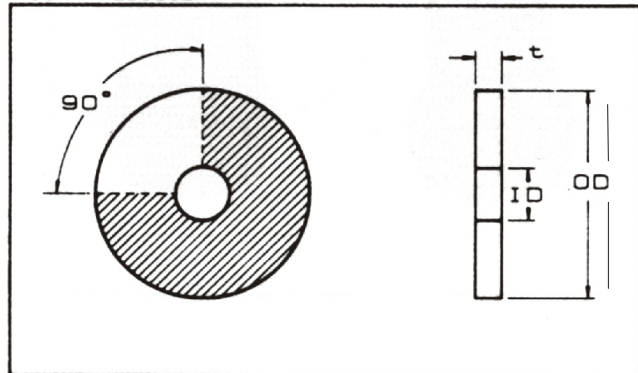
METALLIC CIRCULAR VARIABLE BEAMSPLITTER HIGH PRECISION.
